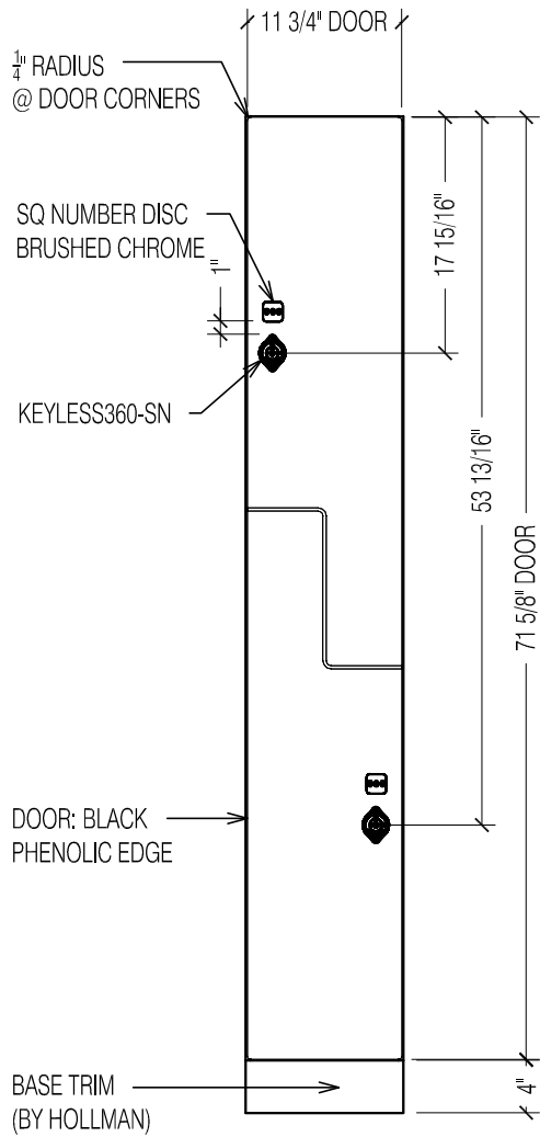
1 FRONT VIEW 3/4" = 1"
