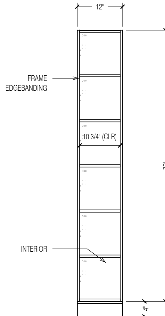
3 OPEN VIEW 3/4" = 1'
